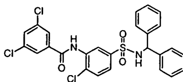
Compound # 52
